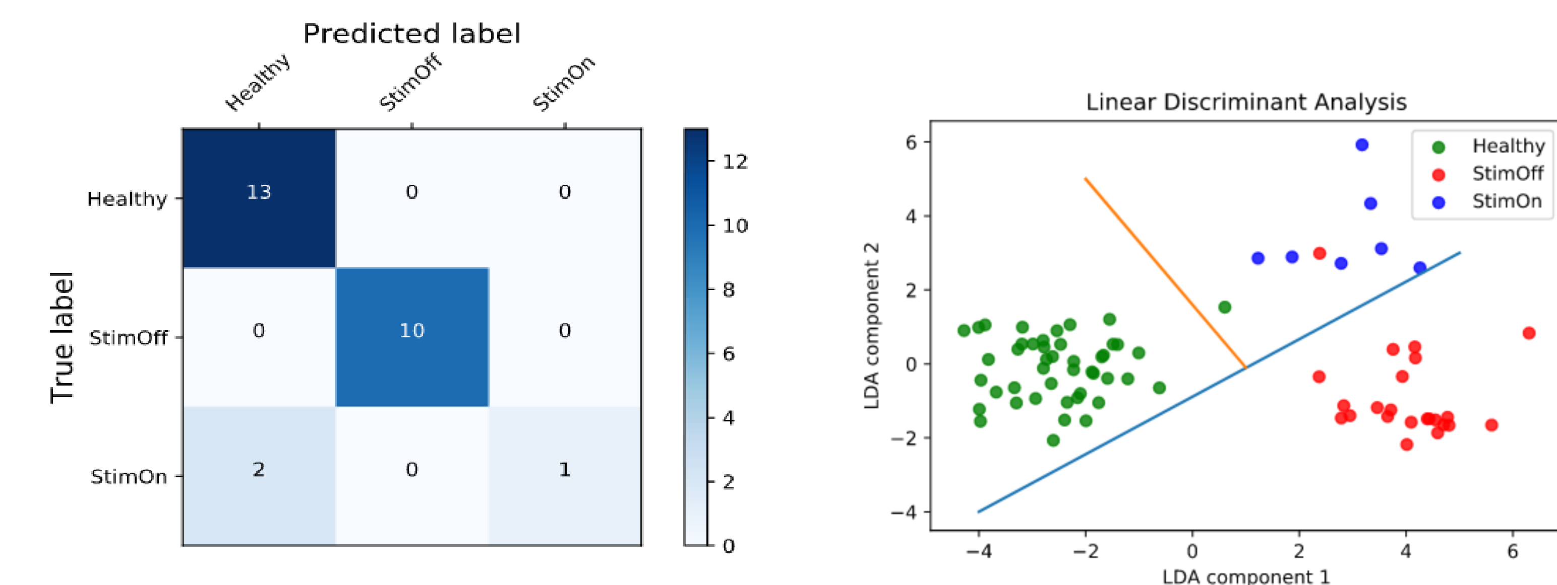
Fig. 5: Classification results, left (confusion matrix of gradient boosting classifier), right (decision boundary of linear discriminant analysis)
